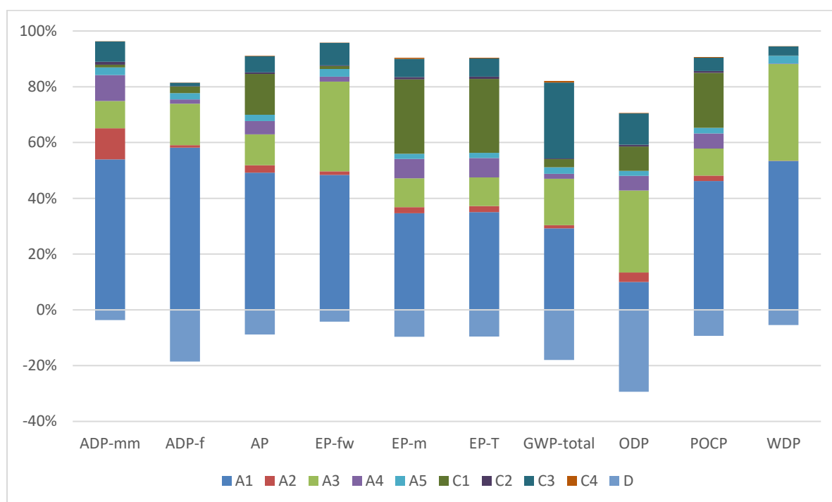
Figure 2: Tensar® RE520 - Impact of the individual modules on the environmental core indicators (NMD set 2)
