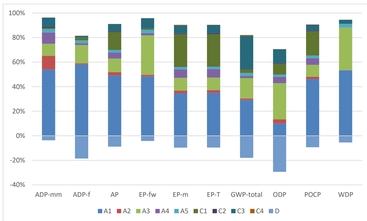
Figure 2: Tensar® RE570 - Impact of the individual modules on the environmental core indicators (NMD set 2)
